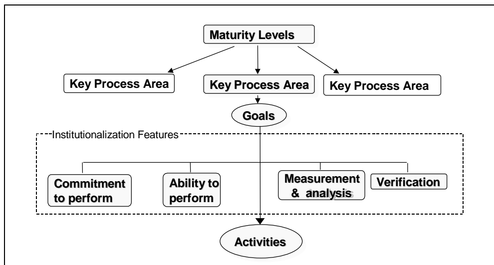
Figure 1. SA-CMM Architecture
